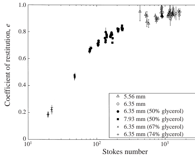
FIGURE 5. Coefficient of restitution, e , as a function of Stokes number for collisions with steel particles on the zerodur wall in water and glycerol–water mixtures.
